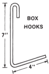
STANDARD BOX HOOKS 5B-6 - 6 Gauge (1/4")
