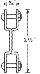
H-50 TWO PIECE BRACKET For hanging loads, hooking in direction of conveyor movement.
