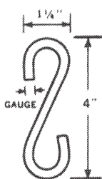
STANDARD "S" HOOKS 4S-6 - 6 Gauge (1/4")
